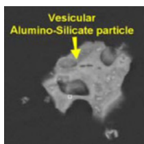
A scanning electron microscopy image with EDS of vesicular almino-silicate provided by RJ Lee.
