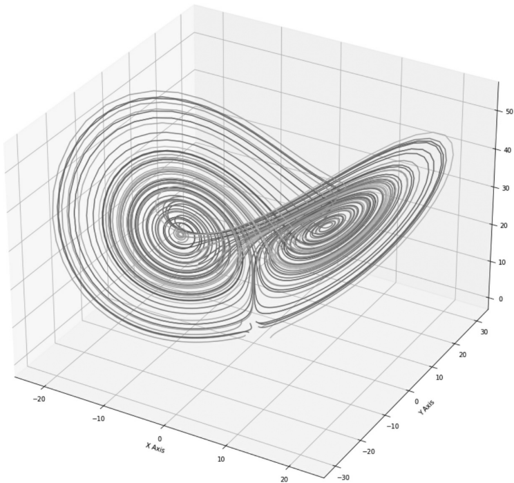
Figure 9.2. The Lorenz attractor
