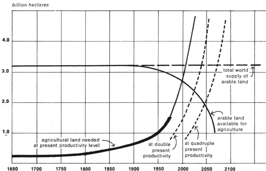
Figure 10 ARABLE LAND
