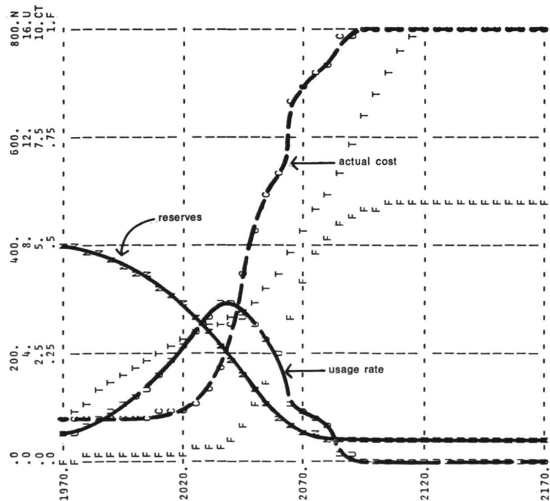
Figure 12 CHROMIUM AVAILABILITY
