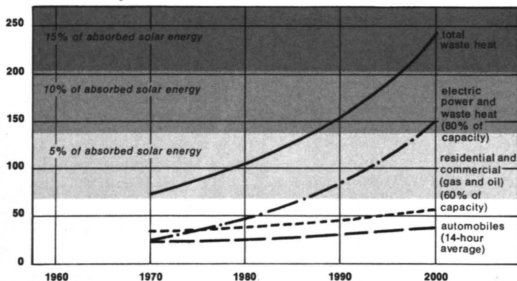
Figure 16 WASTE HEAT GENERATION IN THE LOS ANGELES BASIN
