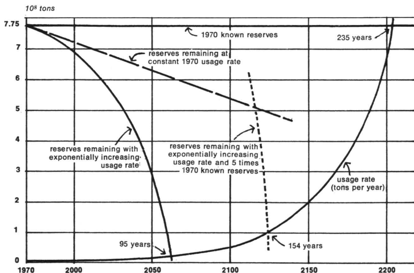
Figure 11 CHROMIUM RESERVES
