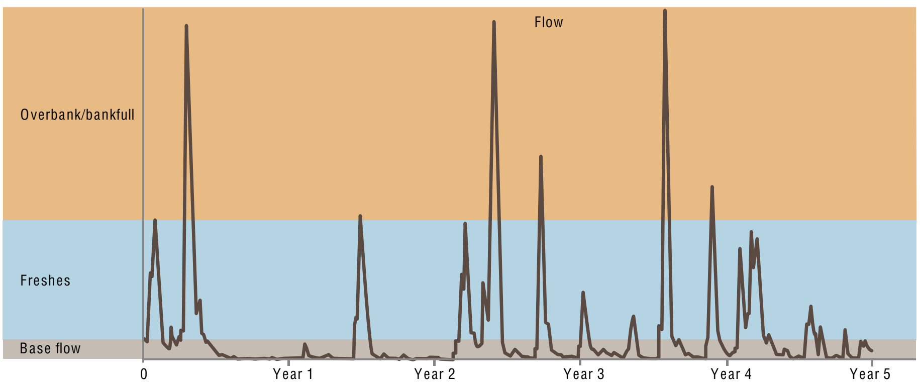
Figure 6.5 Typical flow hydrograph for a river in the northern Basin by water year (July–June)
