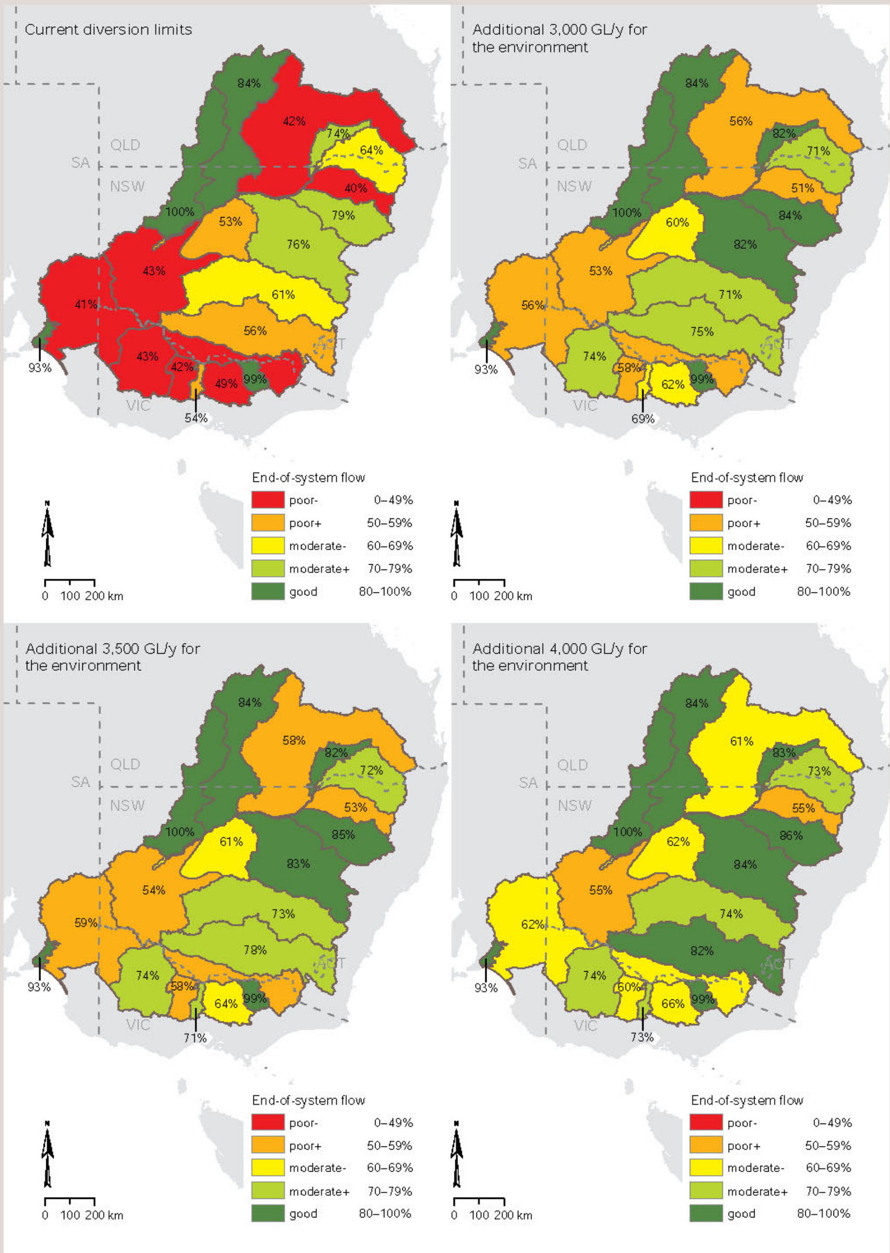
Figure 8.3 Environmental flow outcomes
